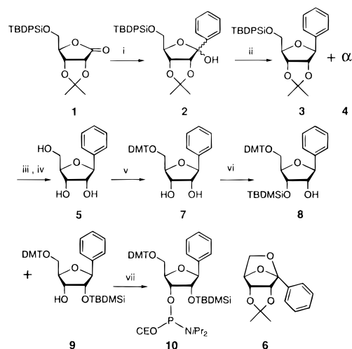
Figure 1. Synthesis of 2'- O - tert -butyldimethylsilyl-5'- O -dimethoxytrityl-3'- O -(2-cyanoethyl N,N -diisopropylphosphoramidite)-1'-deoxy-1-phenyl- \beta -D-ribofuranose. Reagents and conditions: (i) PhLi/THF, -78^\circ\text{C} , (ii) \text{Et}_3\text{SiH}/\text{BF}_3\cdot\text{Et}_2\text{O}/\text{CH}_3\text{CN} , -40^\circ\text{C} , (iii) 1 M TBAF/THF, (iv) 70% aqueous \text{CH}_3\text{COOH} , (v) DMT-Cl/DMAP/ \text{Et}_3\text{N}/\text{Pyr} , (vi) TBDMS-Cl/ \text{AgNO}_3/\text{Pyr}/\text{THF} , (vii) \text{P}(\text{OCE})(\text{N}-i\text{-Pr}_2)\text{Cl}/\text{DIPEA}/1\text{-methylimidazole} .
